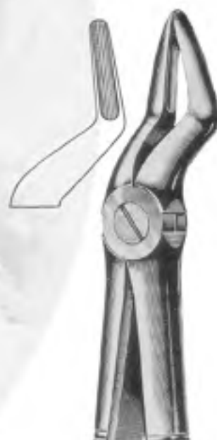
129 Fig.51 Upper roots
