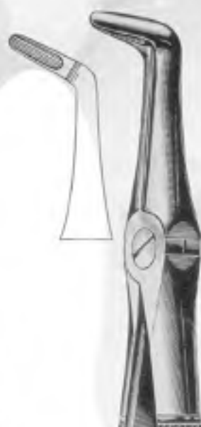
128 Fig.45 Lower roots
