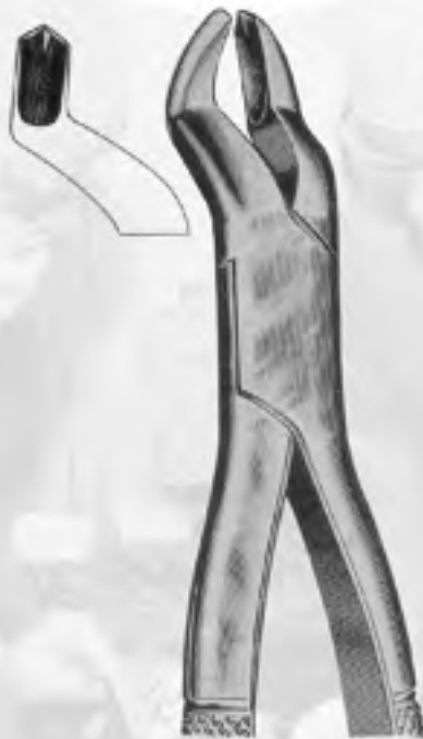
205 Fig. 53 L Upper molars left side
