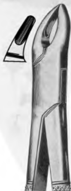
214 Fig. 150 Upper premolars, incisors & roots
